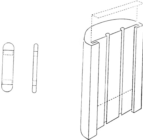
FIG. 231.—Flat metal applicator. Radium is packed in area represented by dotted lines.
